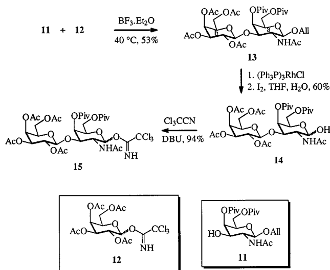
Scheme 3. Synthesis of the Gal \beta (1-3)GalNAc donor 15
