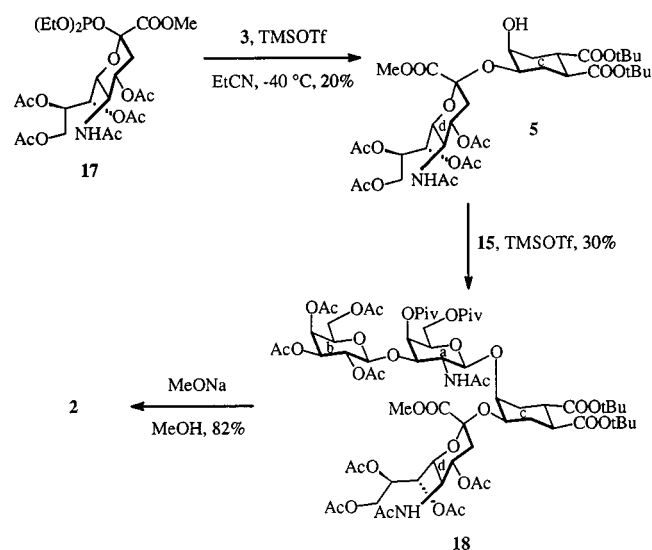
Scheme 5. Route b; synthesis of 2
