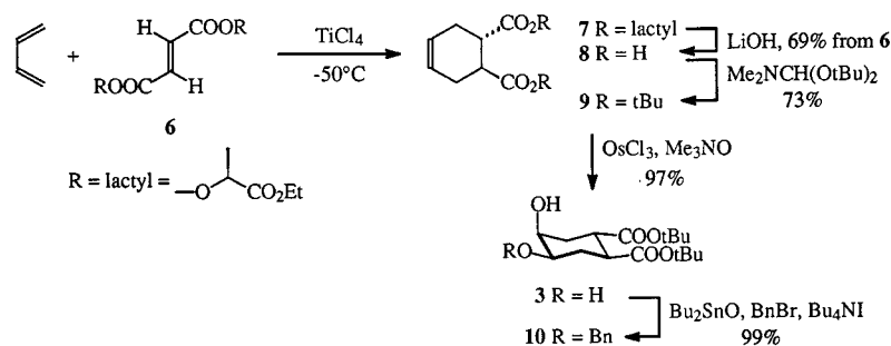
Scheme 2. Enantioselective synthesis of 3
