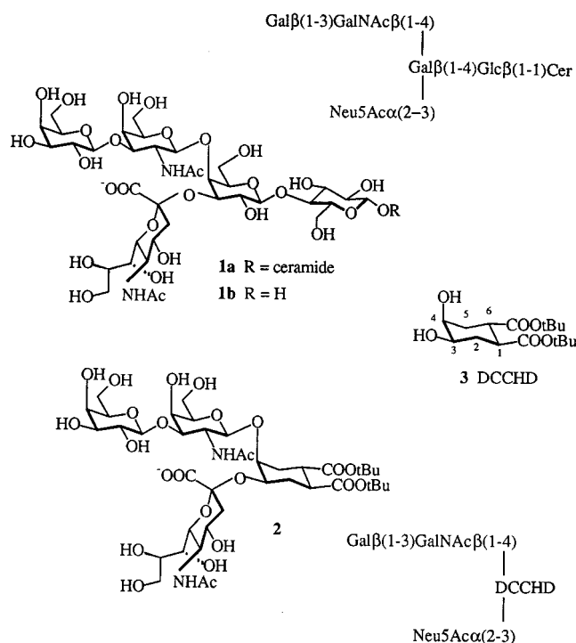
Figure 1. Ganglioside GM1 1 , and its designed mimic 2
